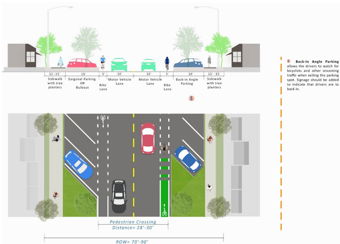
Figure 2.4-B4: Commercial Main Street
