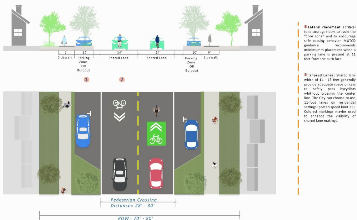
Figure 2.4-26: Collector Street (with shared travel lane)
